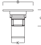
h: 41 mm Alttan ø50 (C3) Bottom ø50 (C3)
